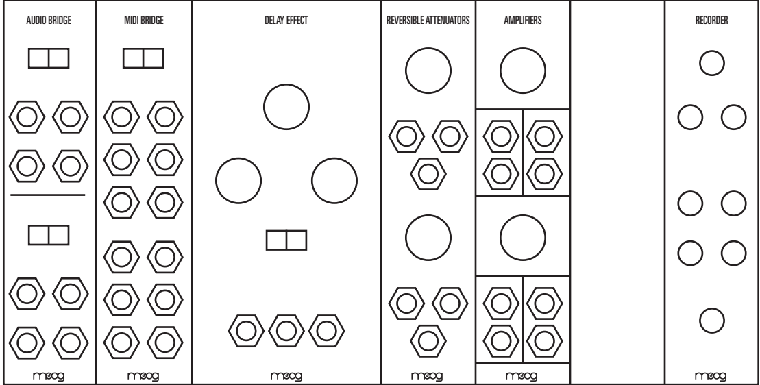
MOOG MODEL 15 SYNTHESIZER
